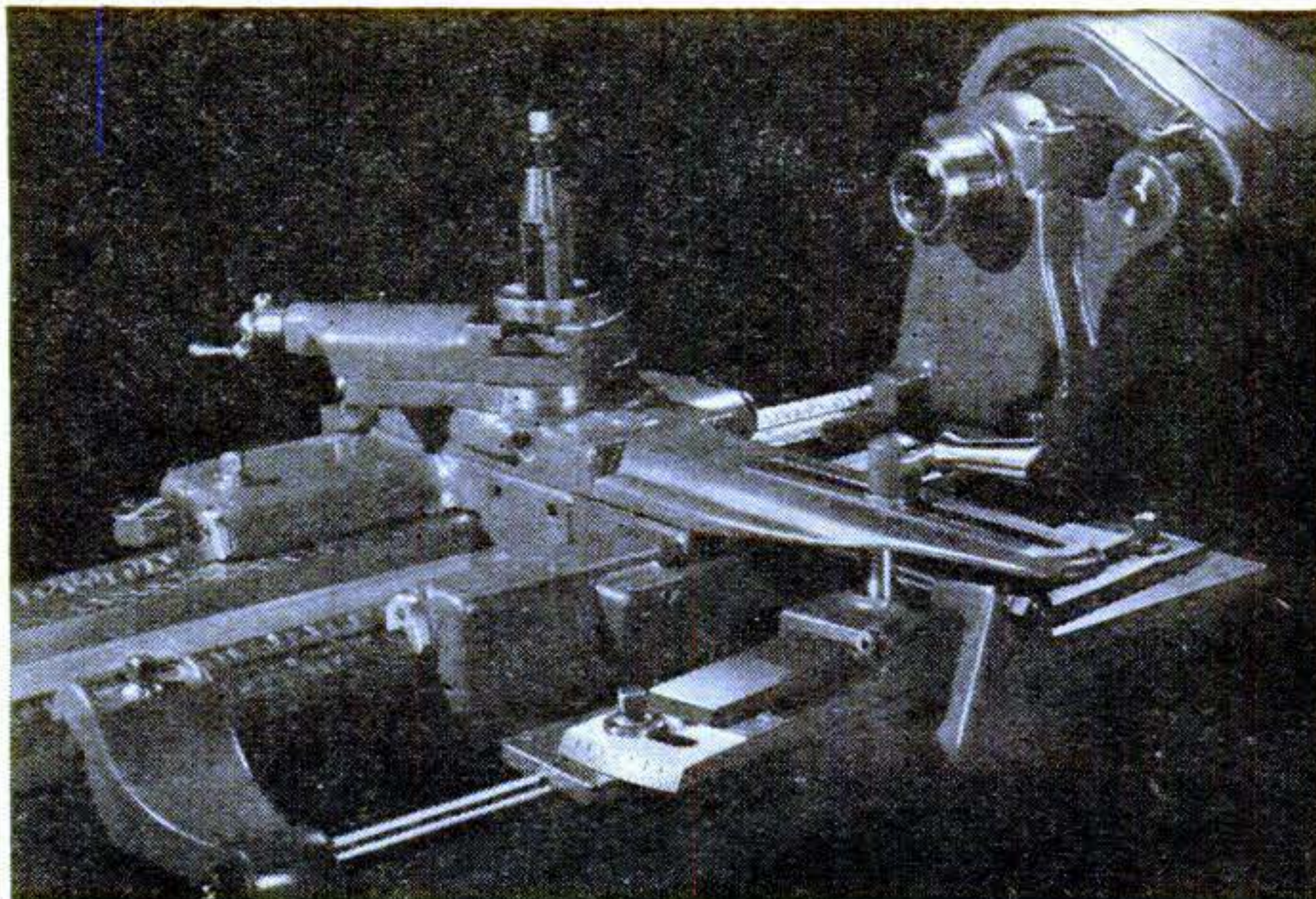
Telescopic Taper Attachment
